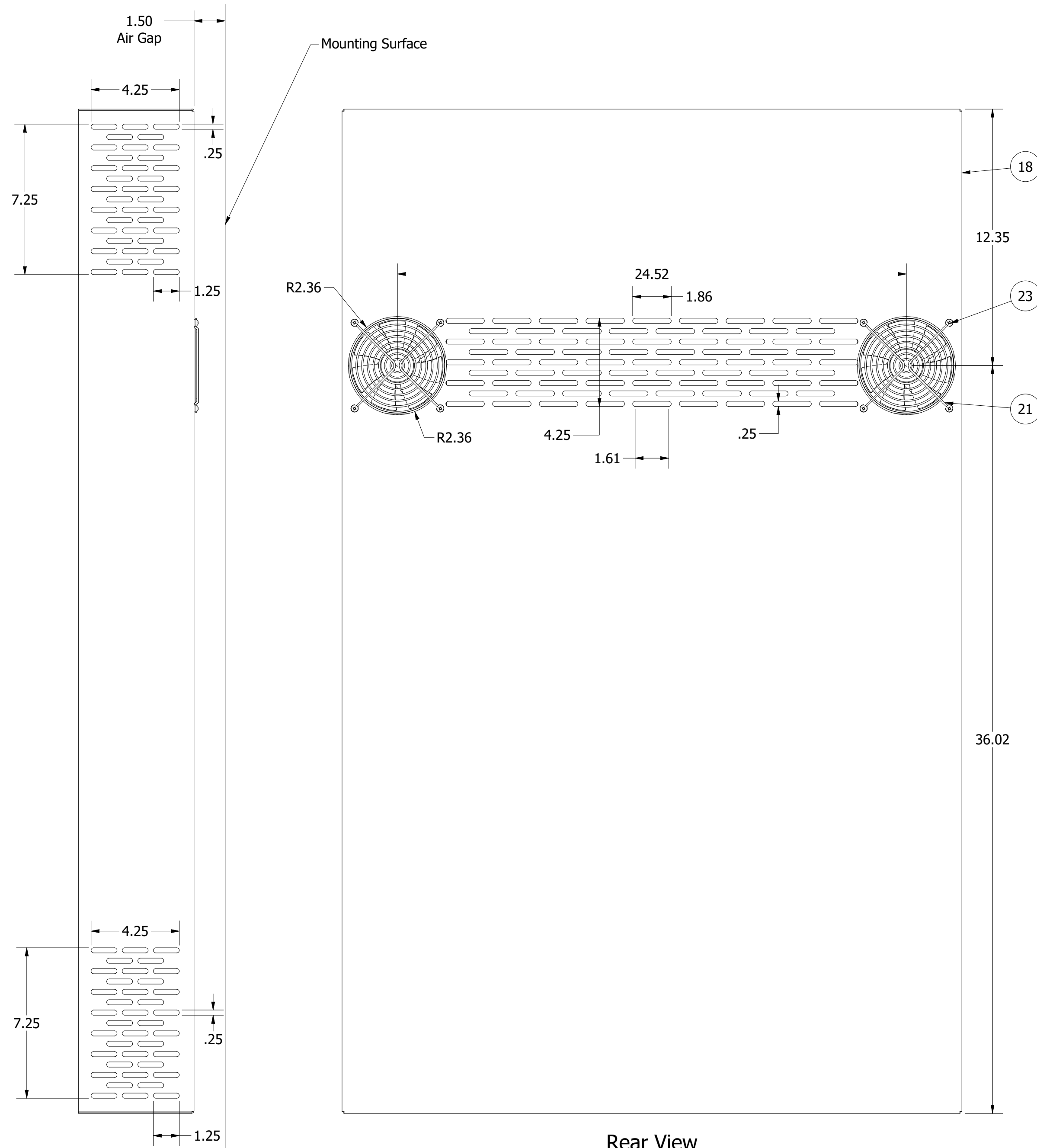
Rear View SCALE 1/4
