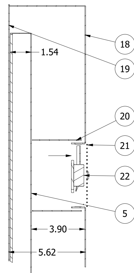
SECTION C-C SCALE 1/4
